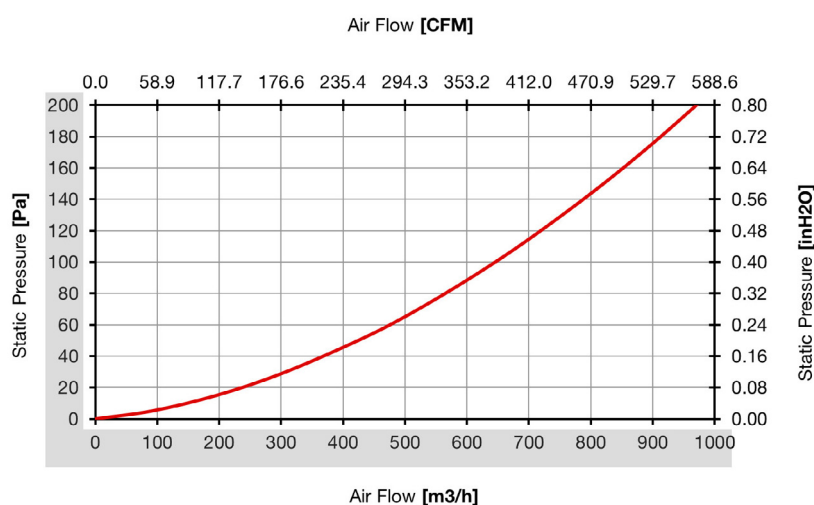
Air performance
