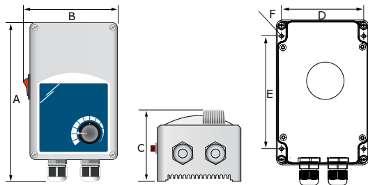
Fig. 1 Mounting dimensions
