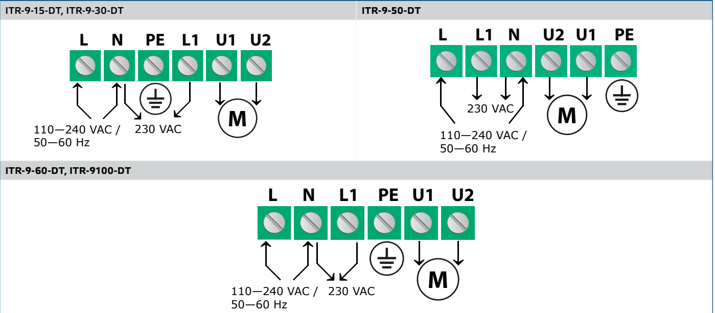
Fig. 3 Wiring and connections
